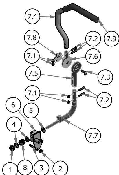
2018 Steering Arm Assembly-Left
