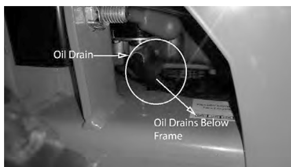
Parts Location
