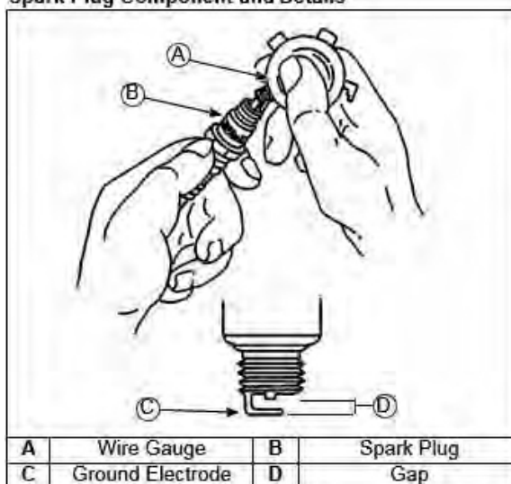
Spark Plug Component and Details
