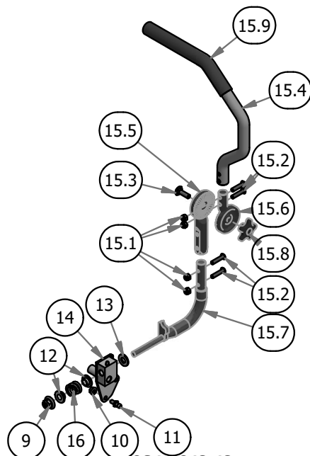
2018 Steering Arm Assembly-Right
