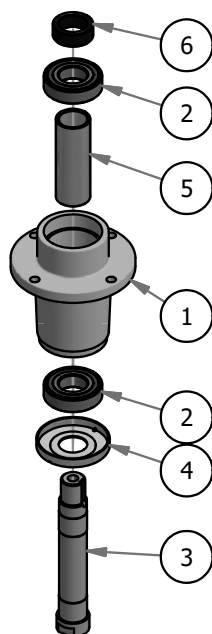
037-6015-50 Spindle- Aluminum -2012 ZT
