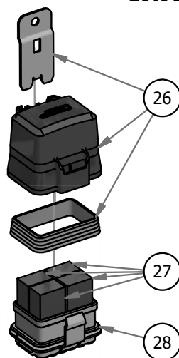
086-3050-19 Wiring Harness
