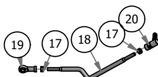
Push Rod-Left
